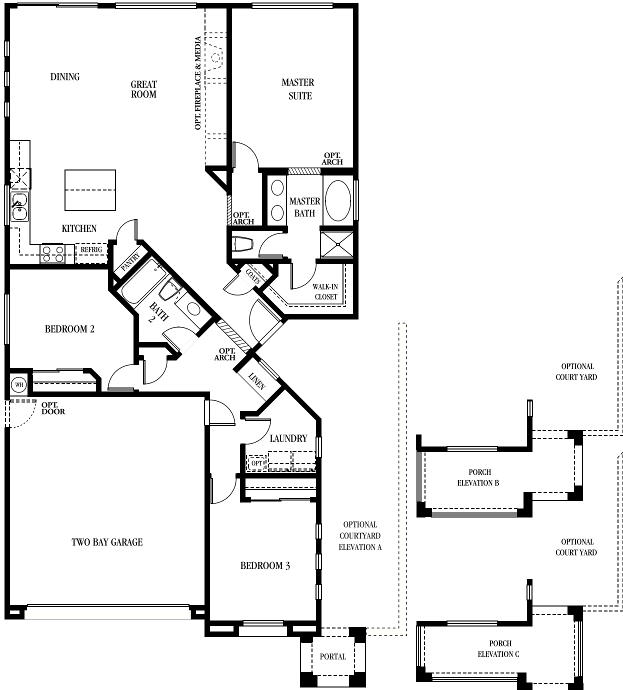
Sierra PLAN 3510 3 Bedroom, 2 Bath, Great Room Courtyard Entry, 2 Bay Garage Approximately 1543 Square Feet
