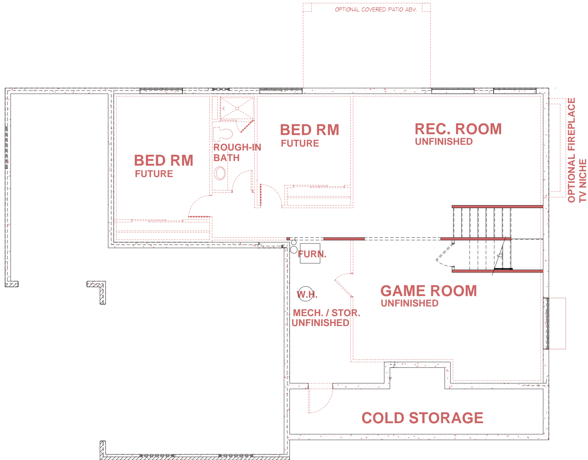
UNFINISHED BASEMENT PLAN
