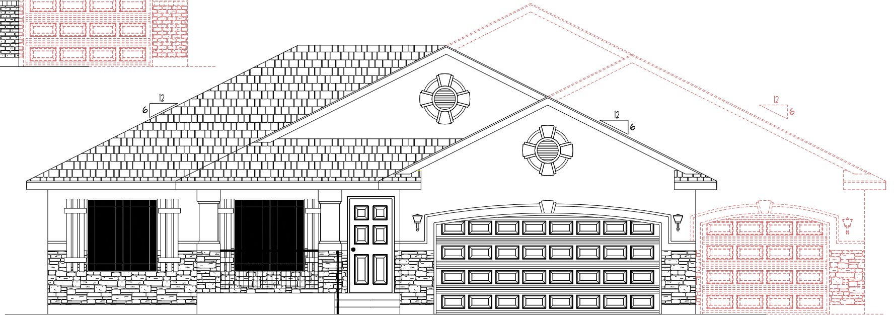
ELEVATION "B"
