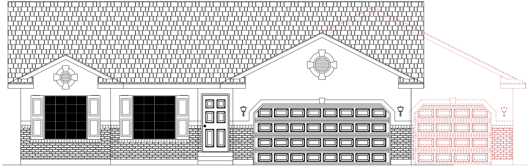
ELEVATION "A"
