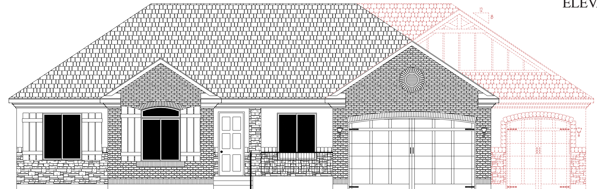
ELEVATION "D"
