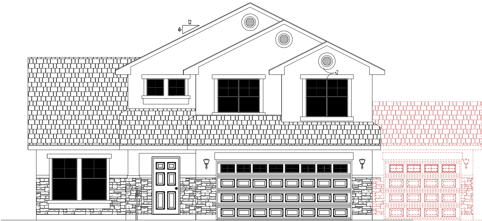
ELEVATION "A"
