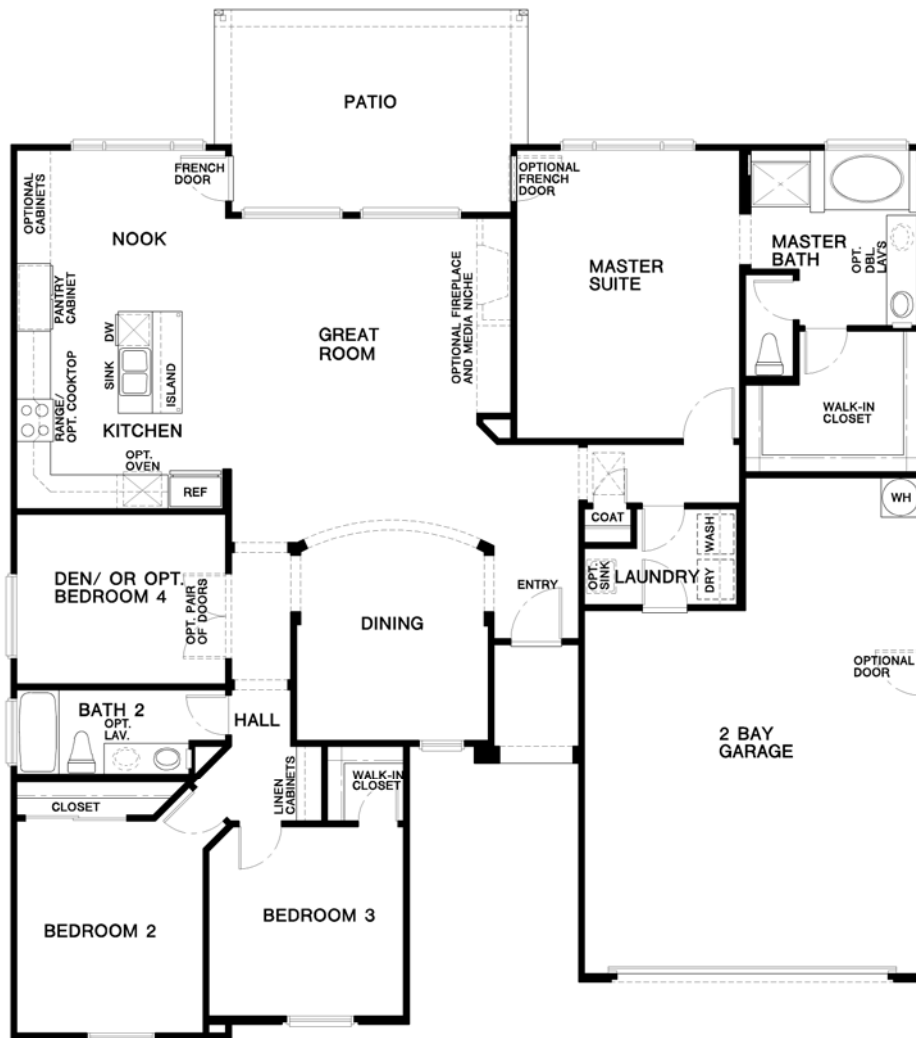
FLOOR PLAN
