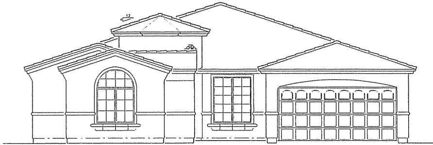
FRONT ELEVATION 'A'
