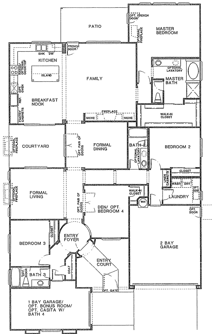
FLOOR PLAN
