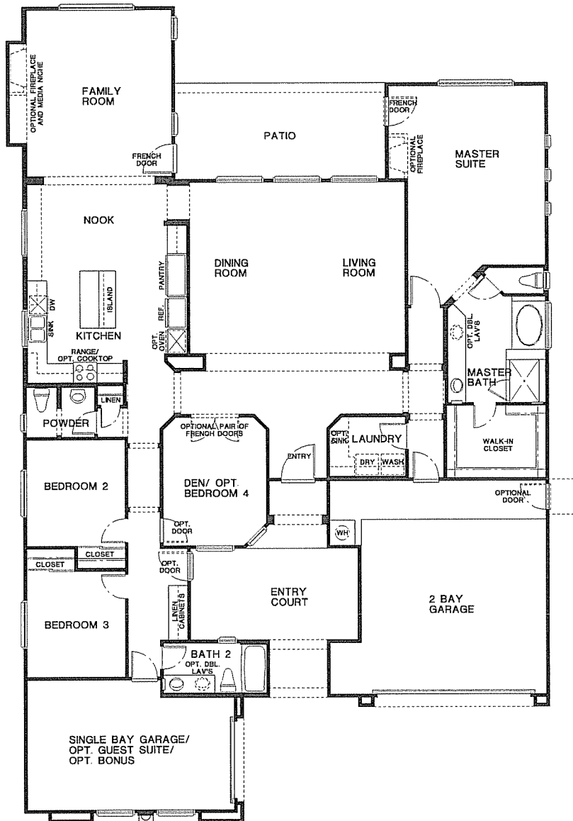
FLOOR PLAN
