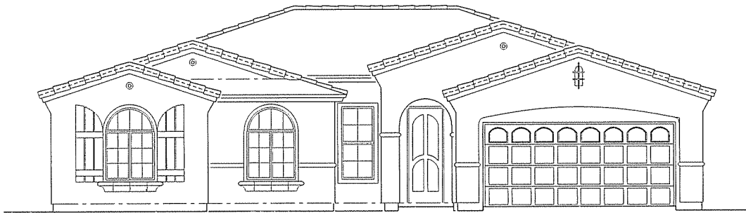
ELEVATION 'A'
